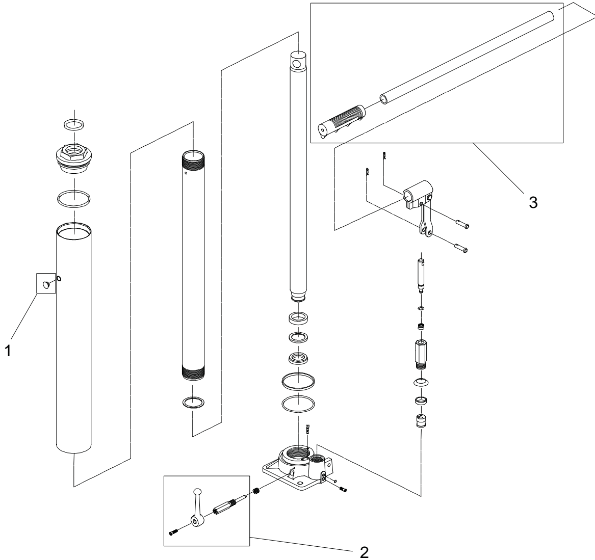
Figure 2 - Replacement Parts Illustration for model ATD-7486
