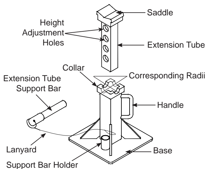
Figure 2 - Model ATD-7449 components
