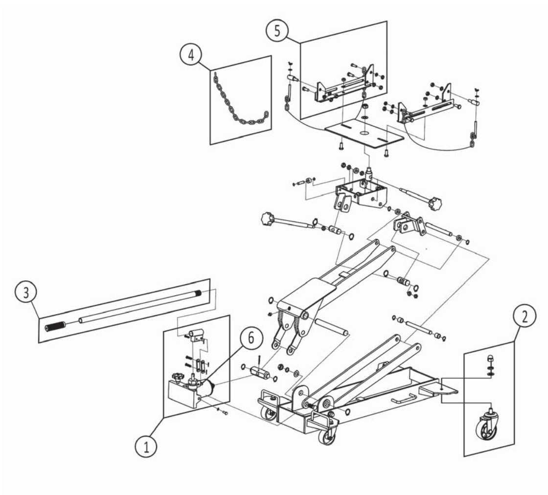
Figure 2 - Replacement Parts Illustration for model ATD-7435A
