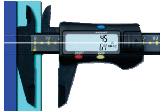
Differential method measurement (Application of zero setting)
