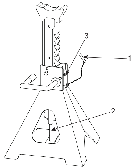
Replacement Parts Illustration for Model Atd-7346 & Atd-7348 (model Atd-7348 shown)
