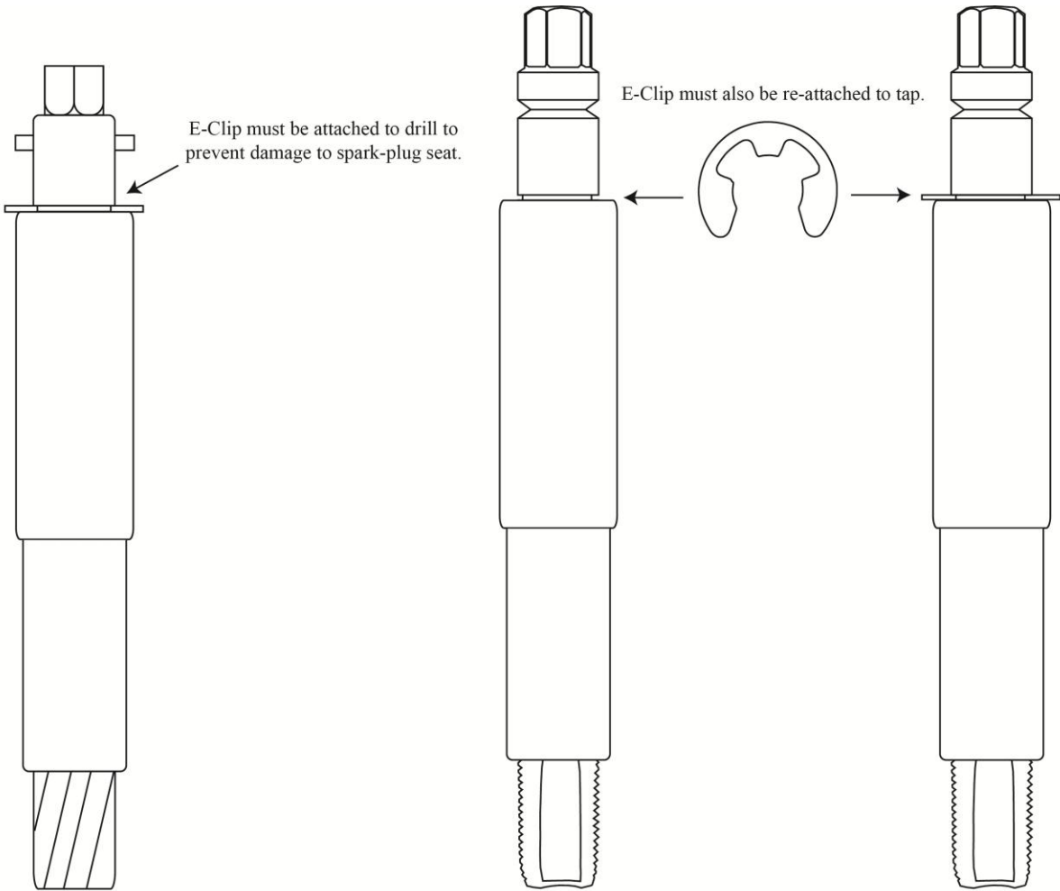
Illustration 1 Core Drill with E-Clip stop in place.
